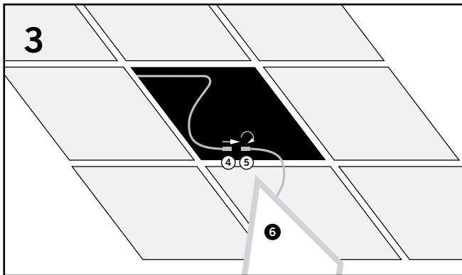
4 - Driver plug lead 5 - Panel plug lead 6 - LED panel
